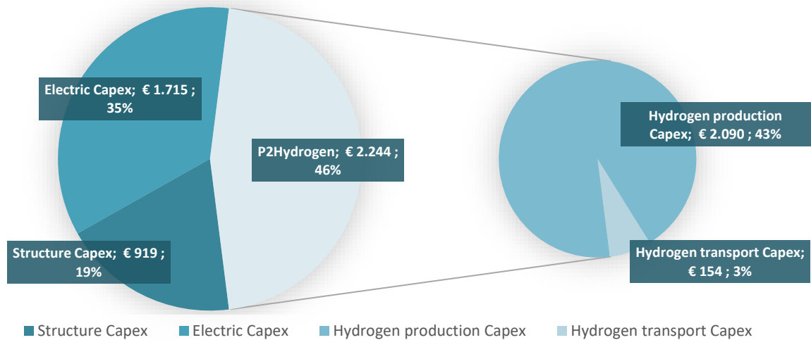
Figure 15 Capex distribution of the 5 GW - 30% scenario
