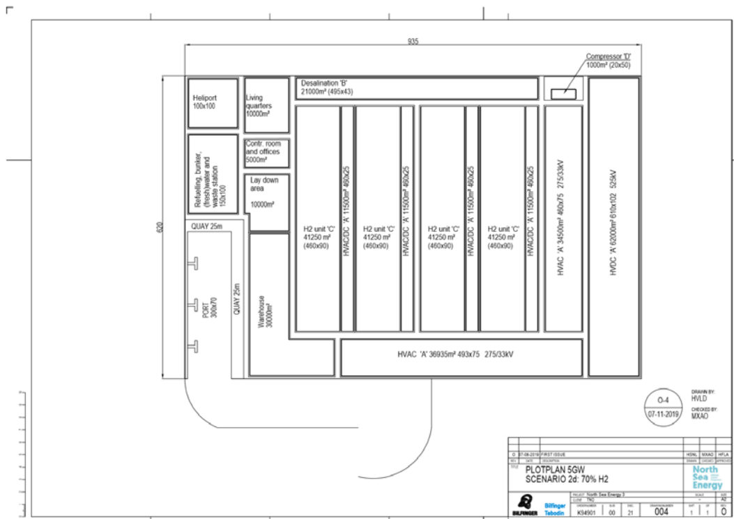
Figure 28 Island Plot Plan Scenario 2d – 5 GW 70% H2 conversion
