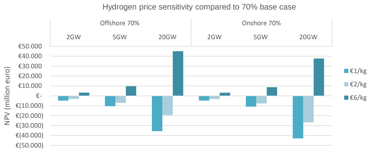
Figure 23: Impact of the hydrogen price for various 70% scenarios in million euros. In the base case the hydrogen price is set at 2 €/kg.
