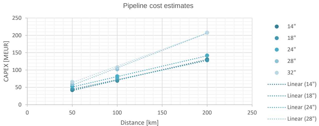
Figure 6 Pipeline cost estimates as a function of diameter and length (author's figure, based on EBN & Gasunie (2018) xiii )
