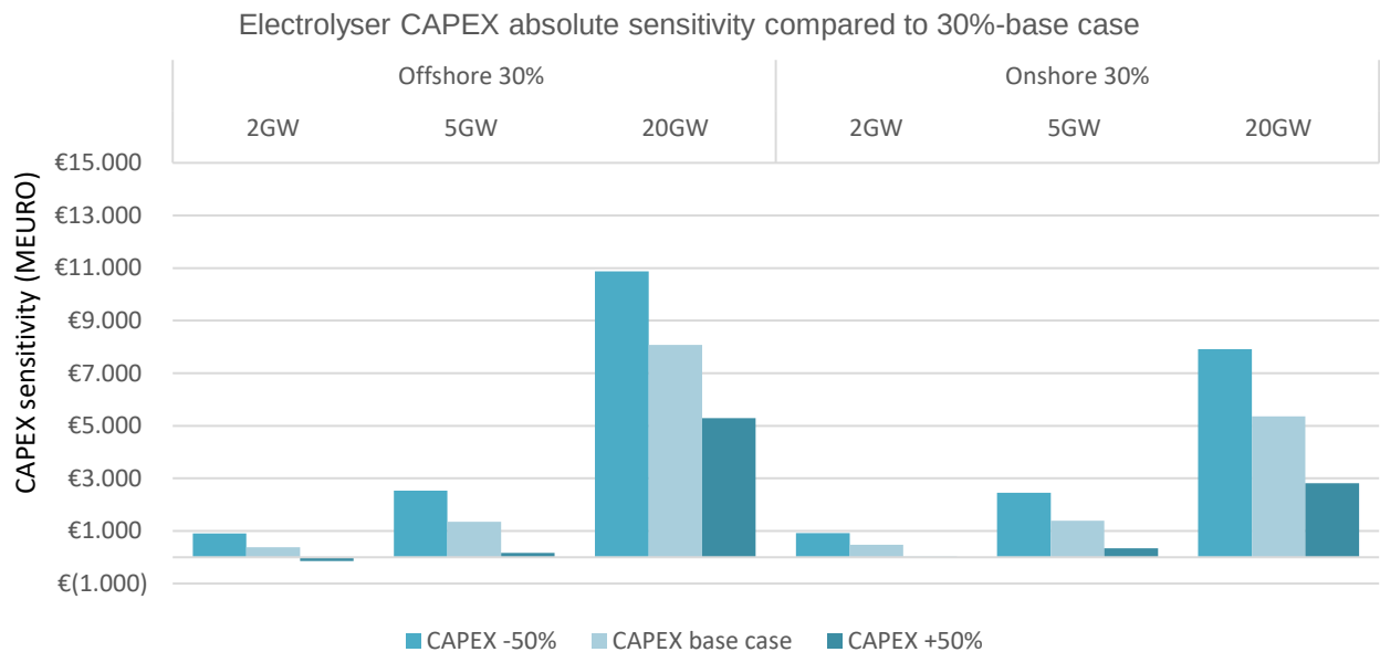
Figure 17 CAPEX sensitivity to electrolyser costs in million euros compared to the 30% hydrogen conversion base case.
