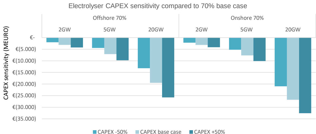
Figure 18 CAPEX sensitivity to electrolyser costs in million euros compared to the 70% hydrogen conversion base case.
