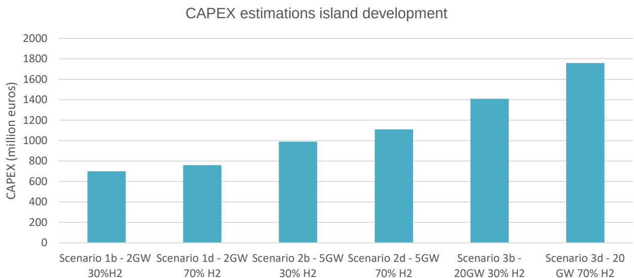
Figure 12 CAPEX estimations for island construction. All estimations are +/- 35% uncertainty. The OPEX are set at a fixed rate of 3 million euros per year with a bandwidth of -25/+100%.
