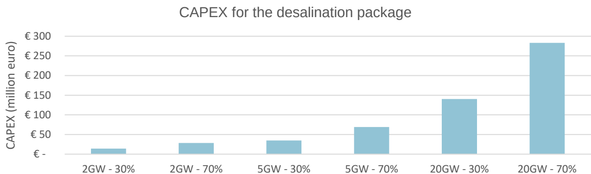
Figure 4 CAPEX desalination package for the various island scenarios
