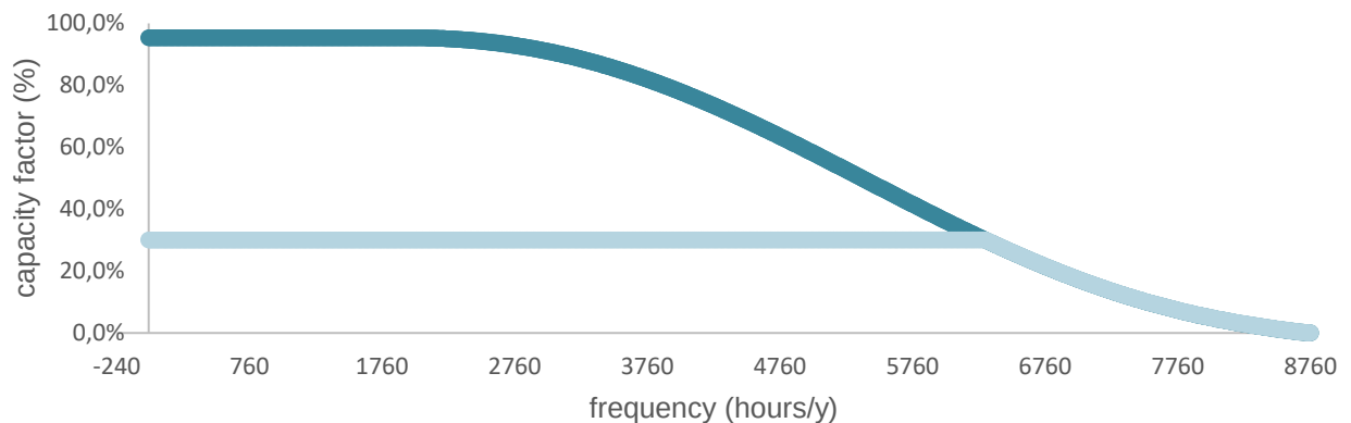
Figure 13 Frequency domain outline of constant production mode (Light blue: wind profile, dark blue: hydrogen profile)
