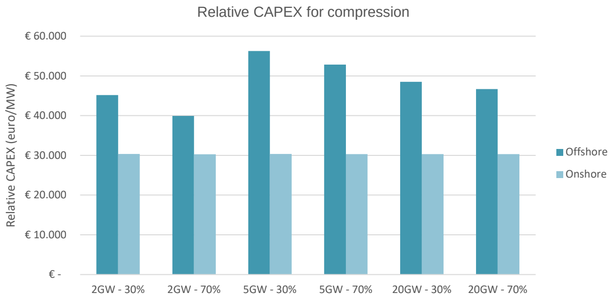
Figure 5 Relative CAPEX of compression in €/MW installed hydrogen capacity
