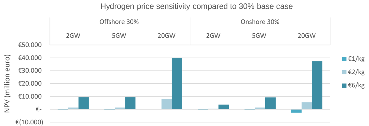
Figure 22: Impact of the hydrogen price for various 30% scenarios in million euros. In the base case the hydrogen price is set at 2 €/kg.
