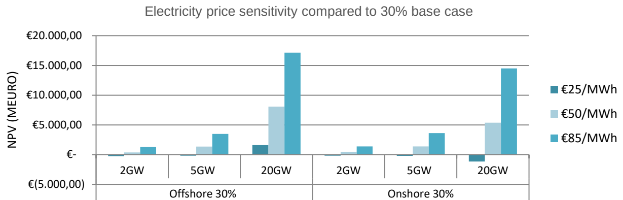
Figure 20 Impact of the electricity price for various 30% scenarios in million euros. In the base case the electricity price is set at 50 €/MWh.
