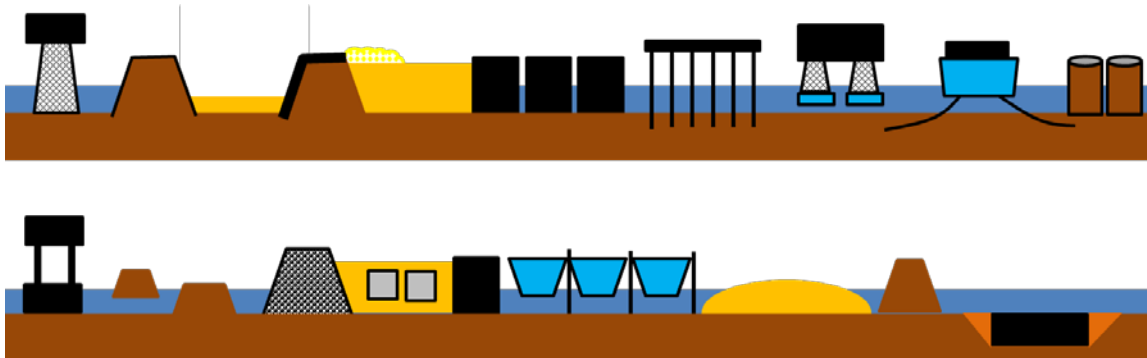
Figure 36 – Different island concepts, ranging from floating, submerged, to polder options (combination of rocks and sand), to a caisson island (picture by Royal HaskoningDHV)
