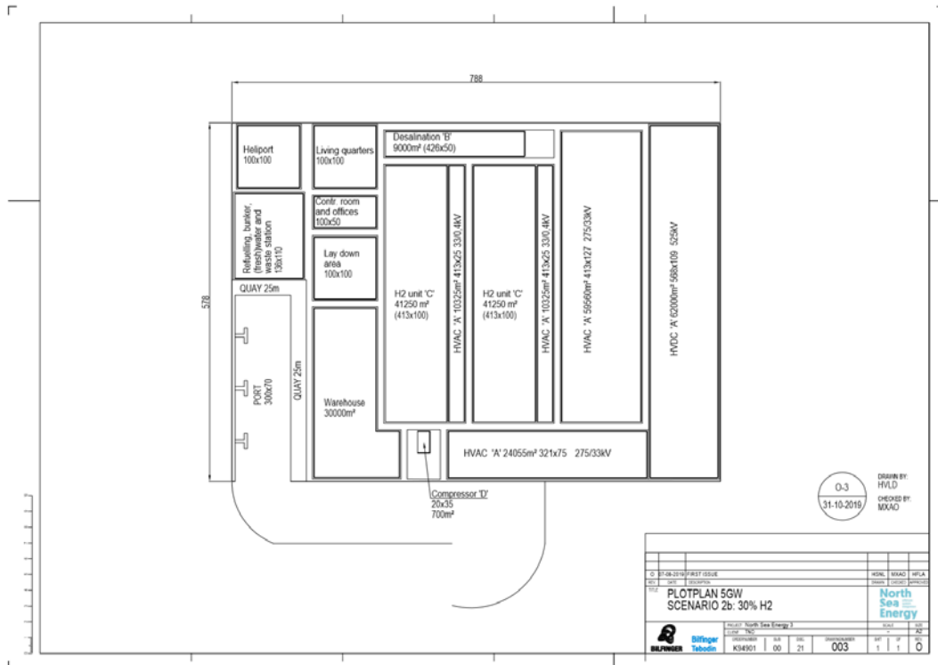
Figure 27 Island Plot Plan Scenario 2b - 52GW 30% H2 conversion
