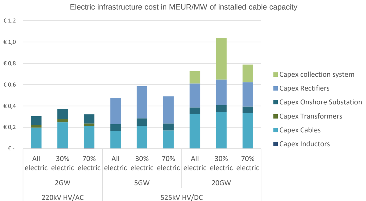
Figure 9 CAPEX costs electric infrastructure per MW of transmission capacity
