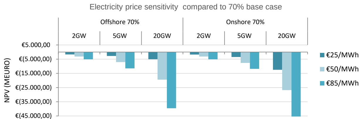
Figure 21: Impact of the electricity price for various 70% scenarios in million euros. In the base case the electricity price is set at 50 €/MWh.
