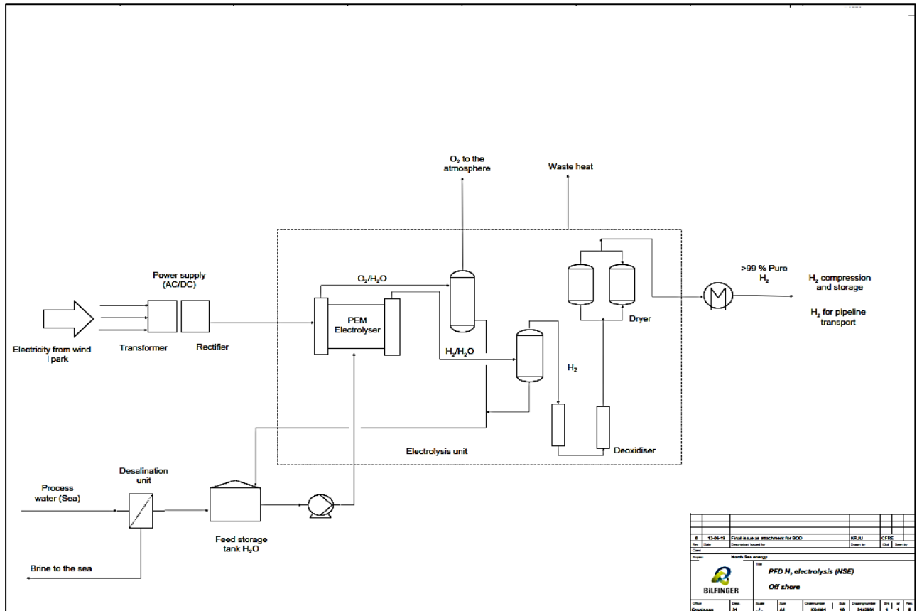
Figure 2 Typical process flow diagram (PFD) for a PEM electrolysis unit
