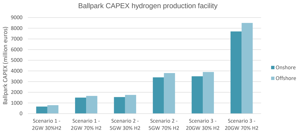
Figure 8 Ballpark CAPEX installation design. The uncertainty in the CAPEX figures is +/-50%.
