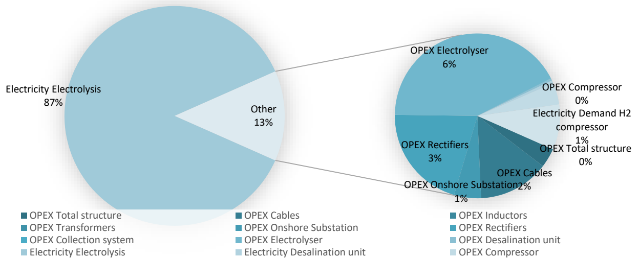
Figure 16 OPEX distribution of the 5GW - 30% scenario
